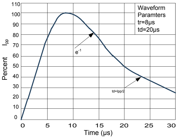
Figure3: Pulse Waveform
