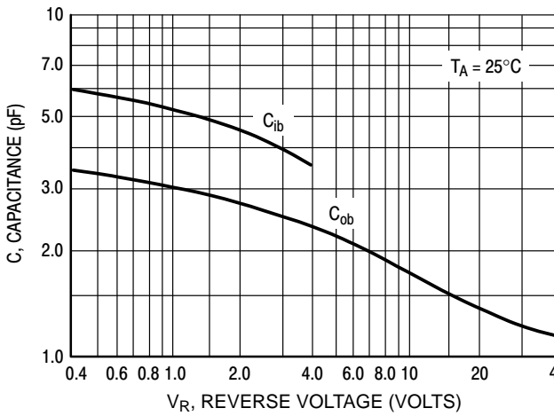
Figure 23. Capacitances
